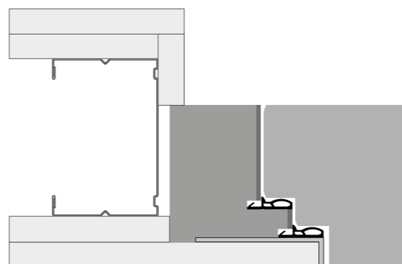
HTBS-8 (wooden frame)
