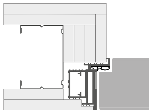
HTBS-4 (aluminum frame)
